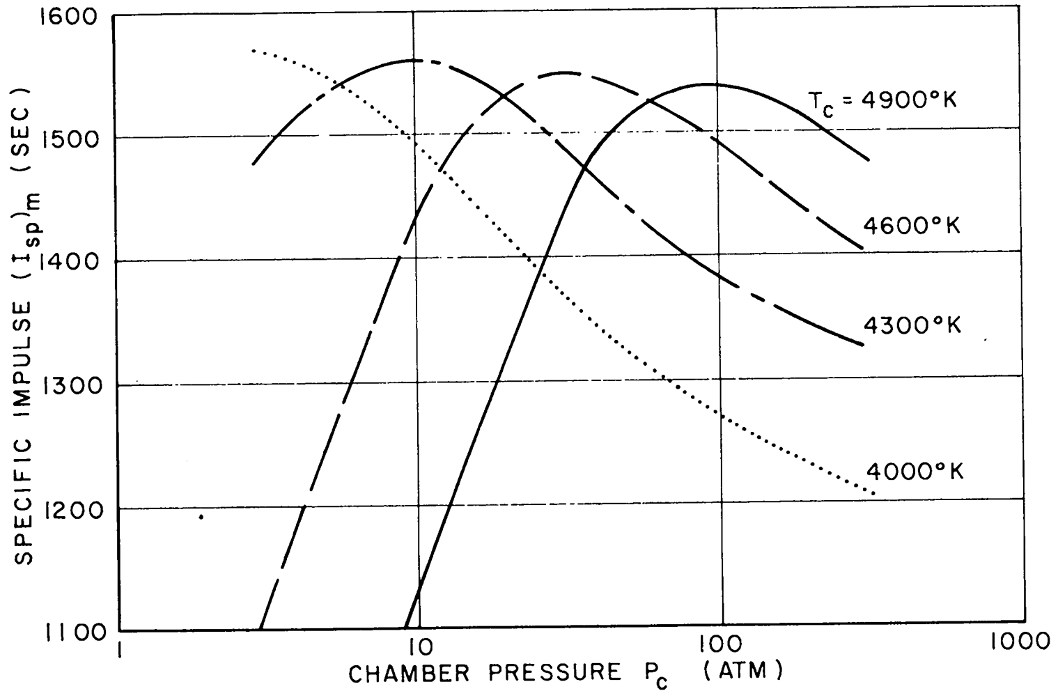
Figure 4. Dependence of Specific Impulse on Chamber Pressure (Dilution Ratio = 1000, Pressure Ratio = 3000)
