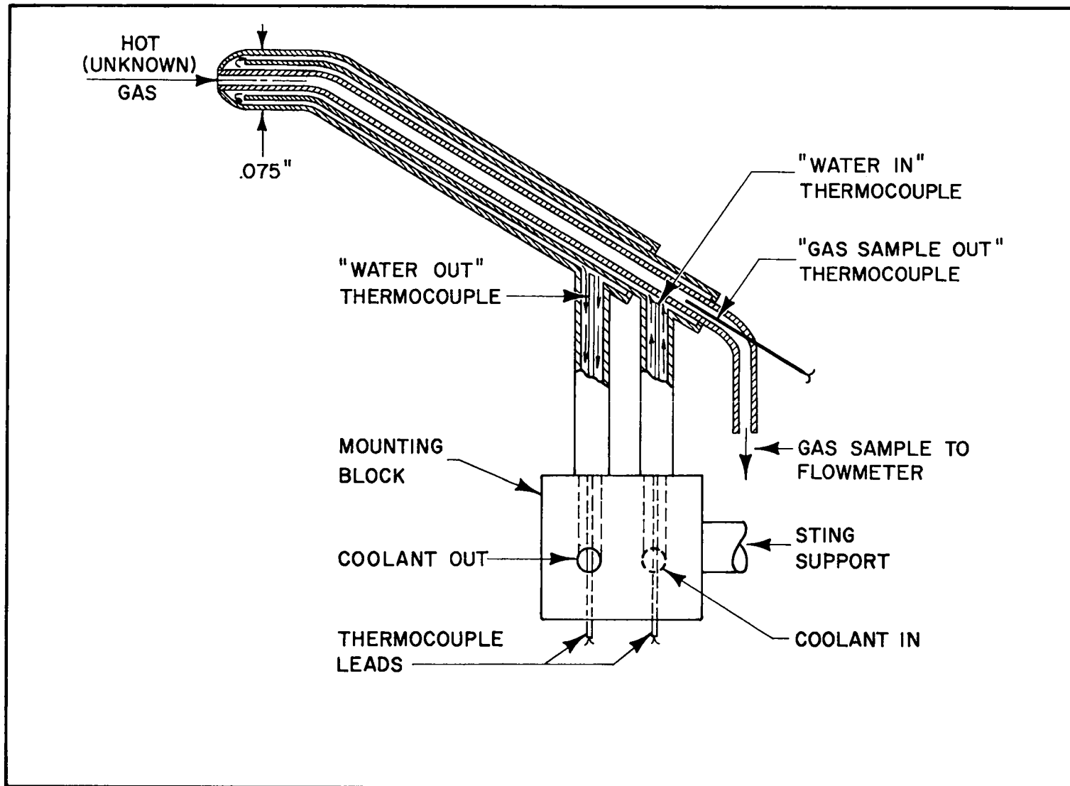
Figure 2. Calorimetric Probe
