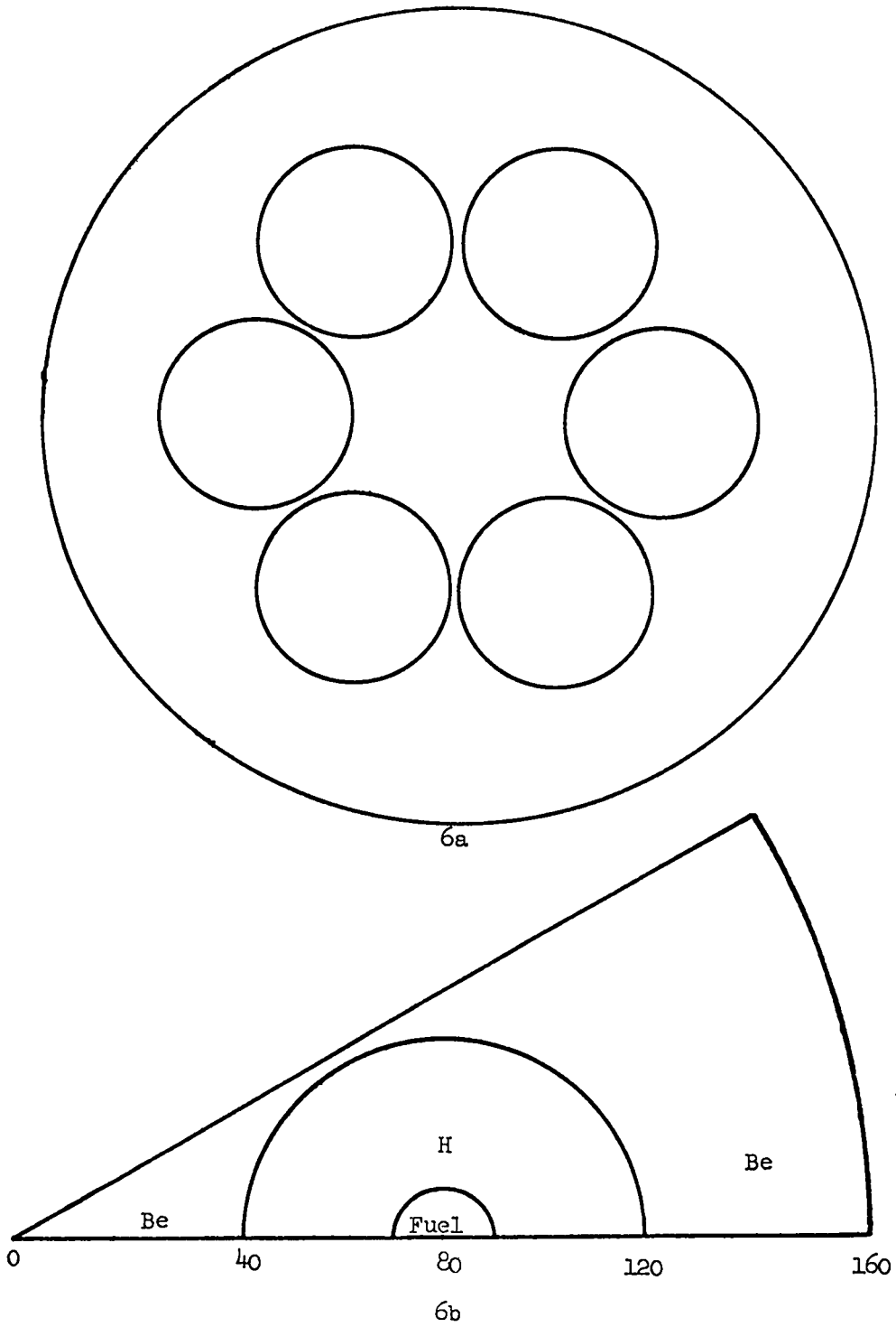
Figure 6. Gaseous Reactor
