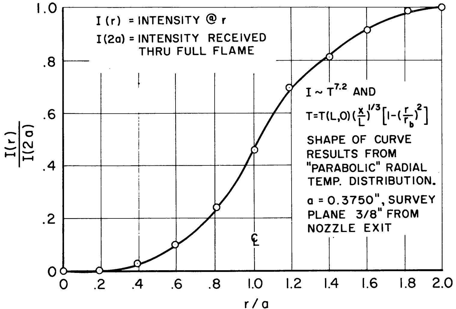
Figure 13. Radial Survey
